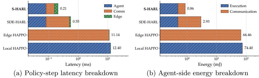
Fig. 4. System cost of S-HARL. By replacing packetized latent delivery with a learned policy message and a short PHY frame, S-HARL removes most of the communication delay and energy incurred by full-stack distributed policy execution.
