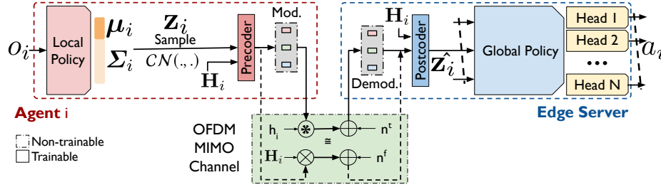
Fig. 2. End-to-end training of S-HARL. The agent-edge interface is inside the policy graph, allowing the local encoders, channel-conditioned precoders/postcoders, global policy, and action heads to be optimized jointly.
