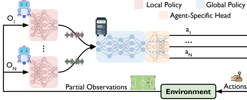
Fig. 1. Overview of S-HARL. Agents encode local observations into semantic policy waveforms conditioned on channel measurements for dynamic data-driven adaptation; the edge aggregates the received latents through a global policy module followed by agent-specific action heads. The actions govern agent behavior and future observations.
