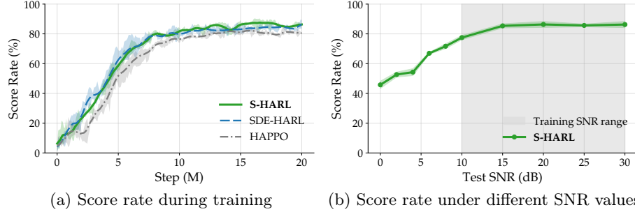
Fig. 3. Policy performance of S-HARL. S-HARL tracks the SDE-HARL baseline during training while using a learned semantic policy signal, and remains robust across the SNR range used during training.
