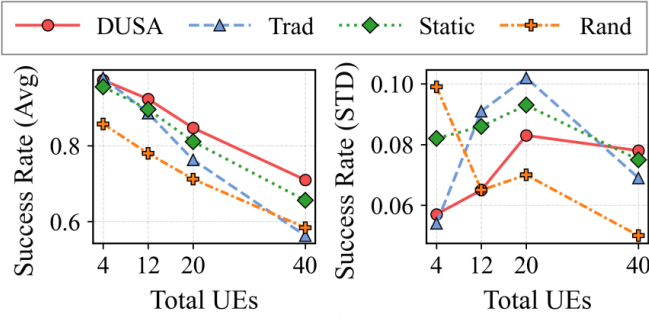
Fig. 3. Average overall UE task success rate vs. total UEs.
