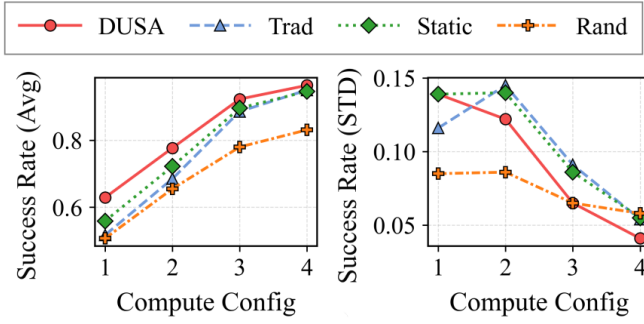
Fig. 5. Average UE task success rate vs. swarm computational budget configuration (x-axis).
