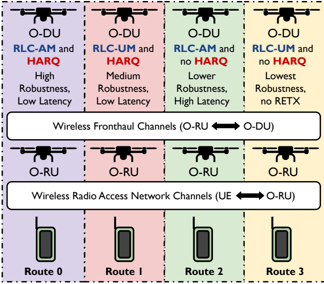
Fig. 2. Semantic O-DU Routes: Route 0 implements both HARQ and RLC retransmissions which enables high-robustness, low latency retransmissions. Route 1 implements only HARQ retransmissions which enables medium-robustness, low latency retransmissions. Route 2 implements only RLC retransmissions which enables lower-robustness, high latency retransmissions. Route 3 does not implement any retransmissions.
