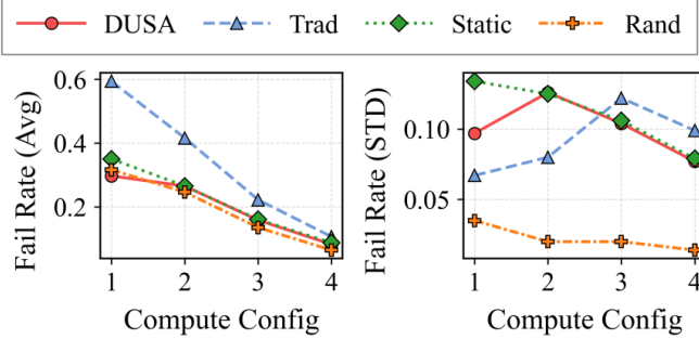
Fig. 6. Average fraction of transmissions where at least one HARQ failure would have occurred vs. swarm compute budget (x-axis).
