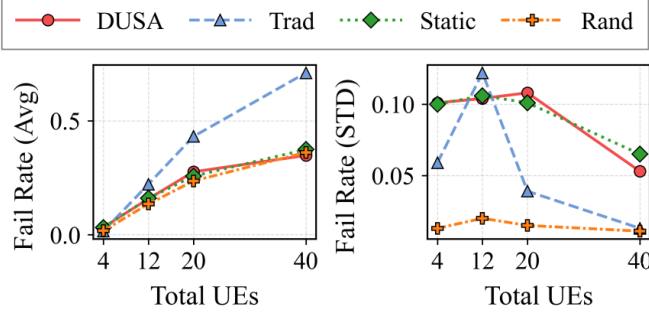
Fig. 4. Average overall fraction of transmissions where at least one HARQ round failure would have occurred vs. total UEs.
