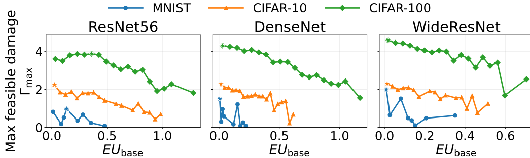
Figure 6: Maximum feasible aleatoric damage as a function of baseline epistemic uncertainty under the standard deep-ensemble uncertainty decomposition. For each dataset and architecture, we bin samples by EU_{\text{base}} and report the upper envelope of feasible damage within each bin. The peak damage typically occurs away from both extremes, corroborating the intermediate-EU vulnerability pattern under the standard expected-entropy / mutual-information decomposition.
