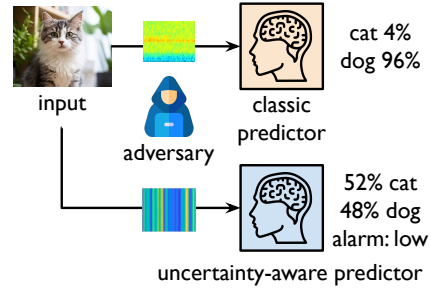
Figure 1: Classical evasion attacks aim to make a predictor confidently wrong; uncertainty-targeted attacks make the model appear legitimately unsure, while the warning signal remains low.
