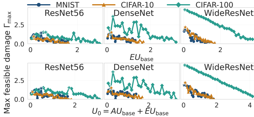
Figure 2: Upper envelope of feasible aleatoric damage across baseline uncertainty budgets. Columns correspond to architectures. The top row bins by baseline EU EU_{\text{base}} , and the bottom row bins by total baseline uncertainty U_0 = AU_{\text{base}} + EU_{\text{base}} . Across settings, the envelope bends and eventually declines rather than increasing monotonically, consistent with the theoretical prediction that the largest feasible damage occurs in an intermediate regime.
