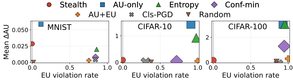
Figure 5: Baseline comparison on ResNet56 across MNIST, CIFAR-10, and CIFAR-100. Each point shows one attack objective, with the x-axis giving the rate of epistemic-stealth violation and the y-axis giving the mean increase in AU. Marker size is proportional to classification accuracy drop. The proposed attack is the only method that stays at zero violation across all three datasets while still producing non-trivial aleatoric damage.
