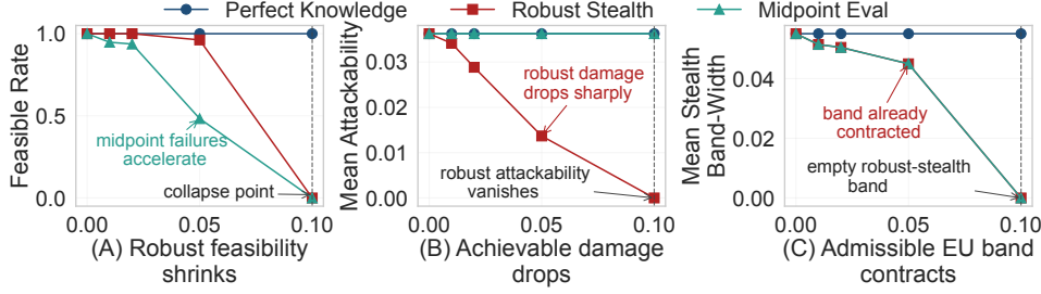
Figure 4: Disclosure-ablation summary on MNIST ResNet56. The x-axis is the attacker’s uncertainty radius r around the baseline epistemic level. Panel (A) shows that midpoint-calibrated attacks begin to fail the robust-stealth test well before complete band collapse. Panel (B) shows that the robust attacker achieves progressively less aleatoric damage than the perfect-knowledge attacker as uncertainty about e grows. Panel (C) visualizes the mechanism directly: the admissible epistemic stealth band contracts with r and eventually becomes empty, at which point robust attackability collapses to zero.
