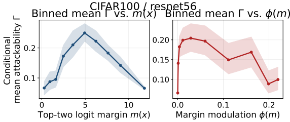
Figure 3: Binned conditional mean attackability \Gamma_{\epsilon,\delta}(x) versus top-two logit margin m(x) (left) and versus the modulation factor \phi(m(x)) (right) for CIFAR-100 / ResNet56. Shaded bands show 95% bootstrap confidence intervals. In this harder setting, the raw-margin relation is non-monotone with a peak at intermediate margins, and the \phi(m) panel similarly concentrates larger vulnerability away from both extremes.
