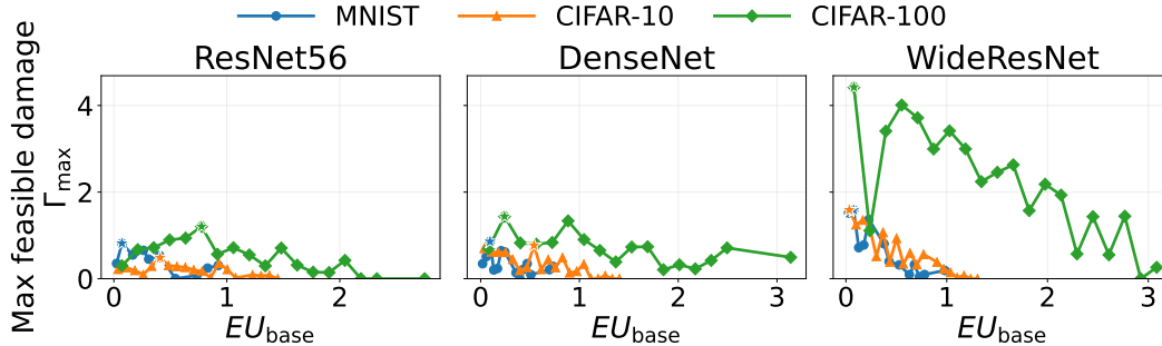
Figure 7: Maximum feasible aleatoric damage as a function of baseline epistemic uncertainty for the label-preserving attack variant. Here the adversarial example is constrained to keep the ensemble prediction unchanged, \hat{y}(\tilde{x}) = \hat{y}(x) . The resulting curves remain non-monotone across datasets and architectures, indicating that the intermediate-EU damage peak is not an artifact of label changes.
