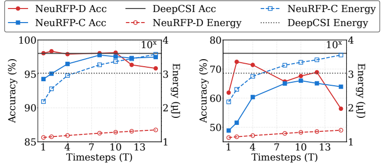
Fig. 4: NeuRFP classification accuracy (left axes) and total analytical energy scaling (right axes, logarithmic) across inference timesteps ( T ), compared against the DeepCSI baseline in (left) Scenario S1, and (right) Scenario S2.
