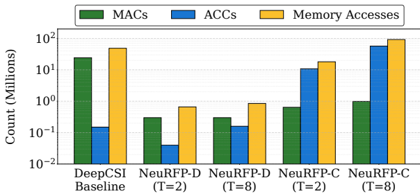
Fig. 3: Comparison of computational operations (MACs, ACCs) and memory accesses among the DeepCSI baseline [8], and our proposed NeuRFP-D and NeuRFP-C architectures at different timesteps ( T ). The plot is in logarithmic scale.
