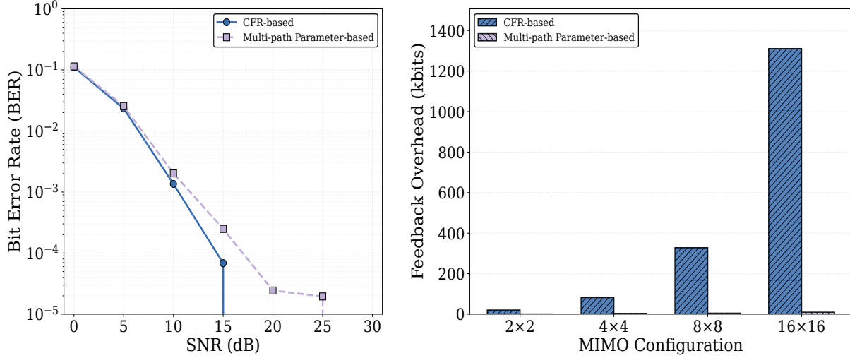
Figure 2. bit error rate (BER) comparison between CFR based feedback and multi-path parameter based in simulation.
